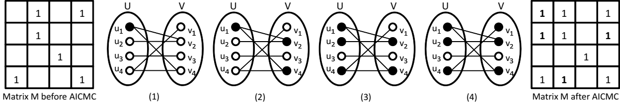
Figure 1: AICMC Example: T is a 4 \times 4 data matrix (not shown) of rank k = 1 . T 's known elements correspond to the positions of the 1s in its visibility matrix M (left side of the figure). The steps of AICMC are: (1) L = \{u_1\} , (2) R = \{v_2, v_4\} , (3) L = \{u_1, u_2, u_4\} , (4) R = \{v_1, v_2, v_4\} . The algorithm stops at the end of (4). The completed elements are (1, 1) , (2, 1) , (2, 4) , and (4, 2) - 1s shown in bold in M (right side of the figure).
